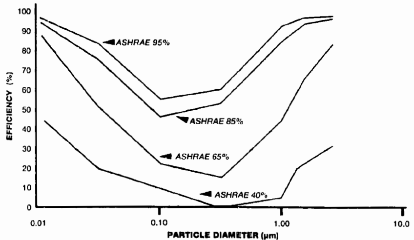
FIGURE 3 PARTICLE SIZE DEPENDENT DRY MEDIA FILTER EFFICIENCIES
